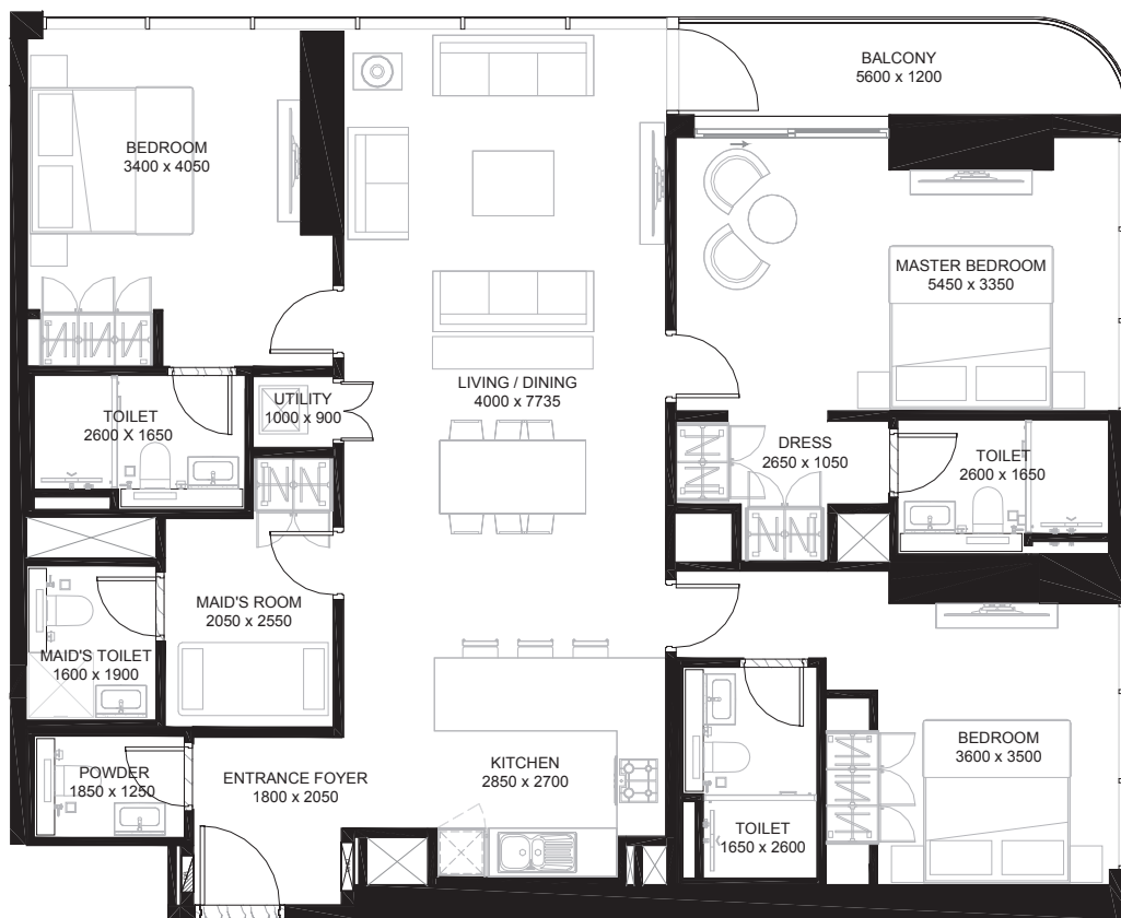
LEVEL 07-28
